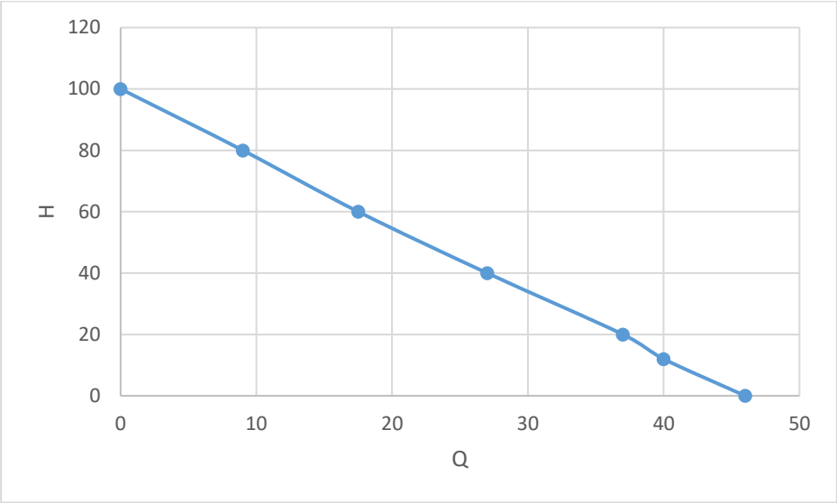
Caracteristica H (m col H2O) – Q (l/ min) a pompei 4KSM 150
