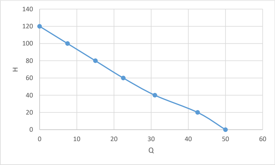
Caracteristica H (m col H2O) – Q (l/ min) a pompei 4KSM 200
