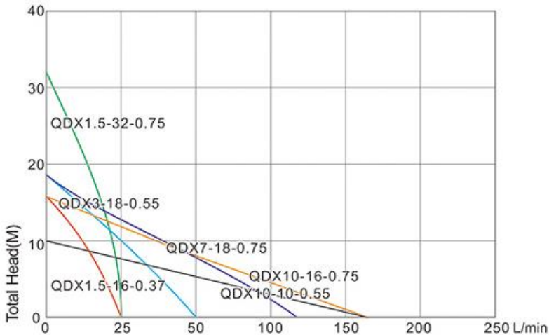
PERFORMANCE CHART AT n=2850r/min
