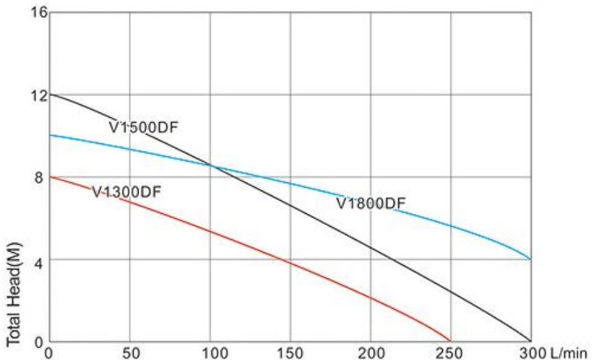
Caracteristica H (m col H 2 O) – Q (l/ min) a pompei V1300DF PERFORMANCE CHART AT n=2850r/min
